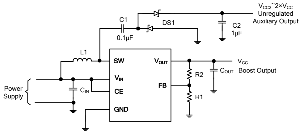
Figure 21. Power Supply Solution With Auxiliary Positive Output Voltage
